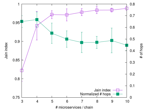
Figure 2: Load balancing and hops vs. chain length L_c
