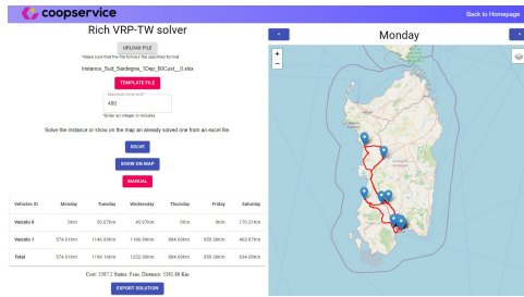
Figure 4: A screenshot of the MTVRPTW module.
